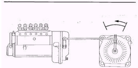
Figure 2 Fuel Control Lever at Mid Fuel Position
