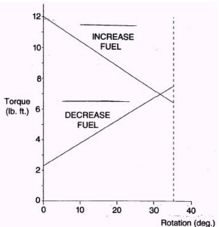
Figure 1 Actuator Torque
